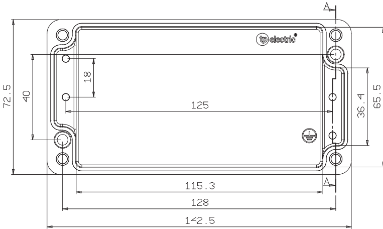
Gövde / Housing
