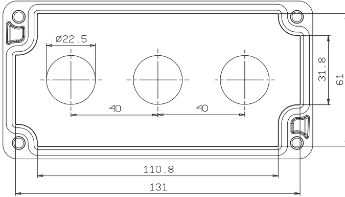
Kapak / Cover
