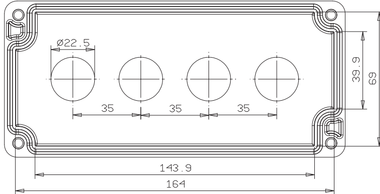
Kapak / Cover
