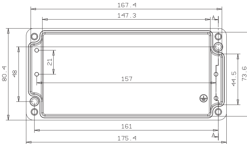
Gövde / Housing
