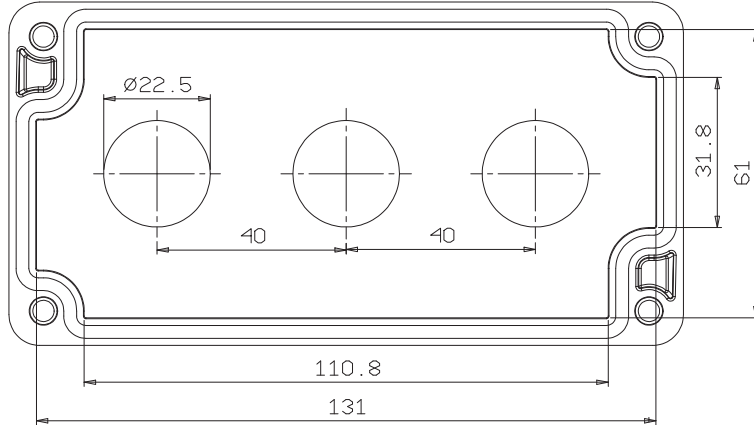
Kapak / Cover
