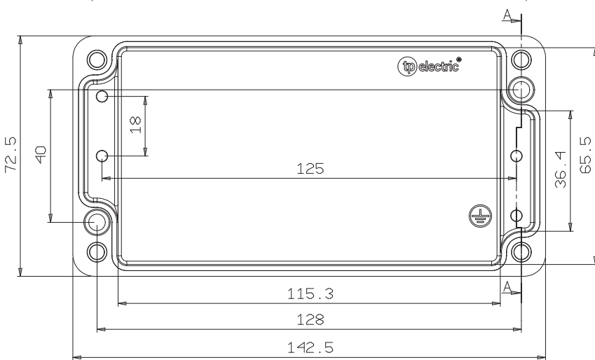
Gövde / Housing
