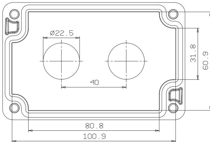
Kapak / Cover
