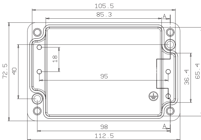
Gövde / Housing
