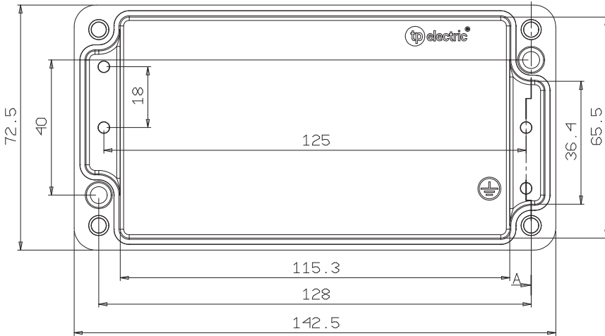
Gövde / Housing
